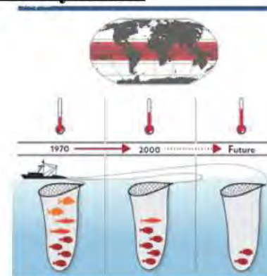
Figure 3.11.7 Average mean temperature of catch (MTC) and sea surface temperature (SST) from (upper) non-tropical and (lower) tropical large marine ecosystems (left panels). The right panels are schematic representation of hypotheses explaining the change in MTC over time (from Cheung et al. , 2013a).
