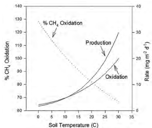
Figure 3.4.4 A model illustrating the potential for \text{CH}_4 oxidation to decline as a fraction of methane production with increasing temperature (Megonigal, 1996).
